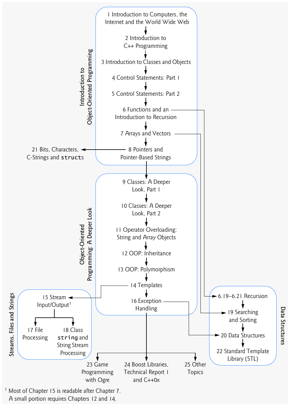
Fig. 1 | C++ How to Program, 6/e chapter dependency chart.
